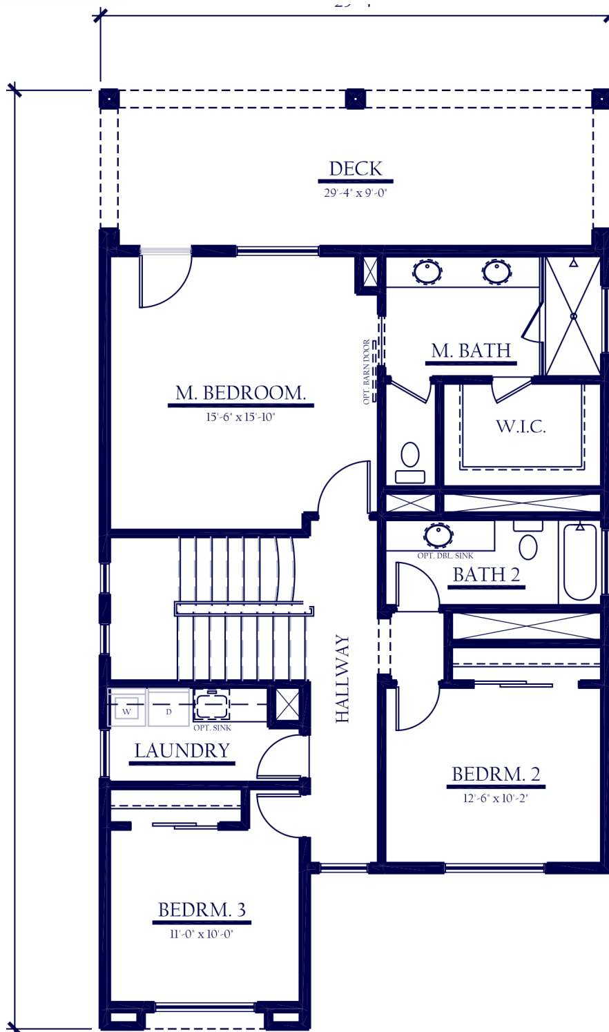
UPPER FLOOR PLAN 2887
