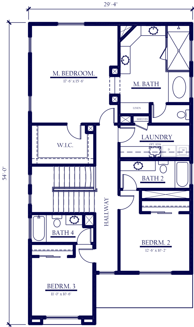
ALTERNATE UPPER FLOOR PLAN ENSUITE OPTION
