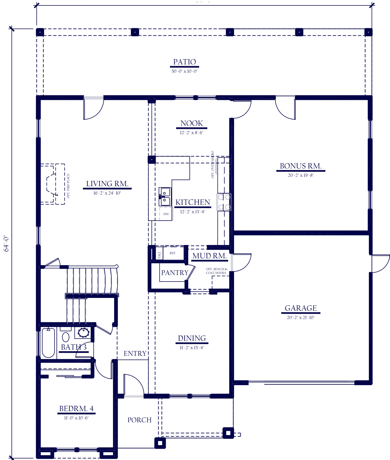
FIRST FLOOR PLAN 2887
